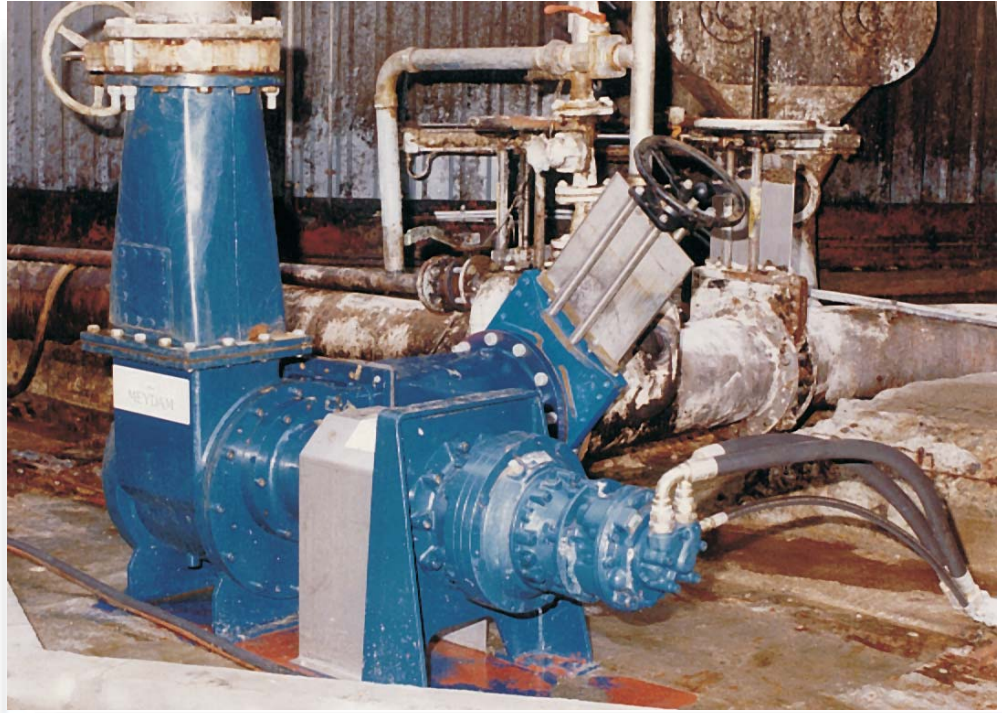
Meydam MTP35 - Silfas Egersund - Pumping from storage to cooker.
