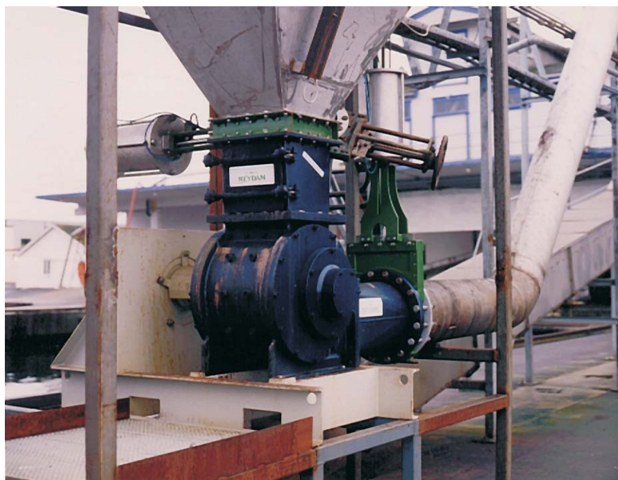
Meydam MTP45 - Installation at Silfas Egersund AS- Norway Pumping dewatered fish from weight system to storage.
